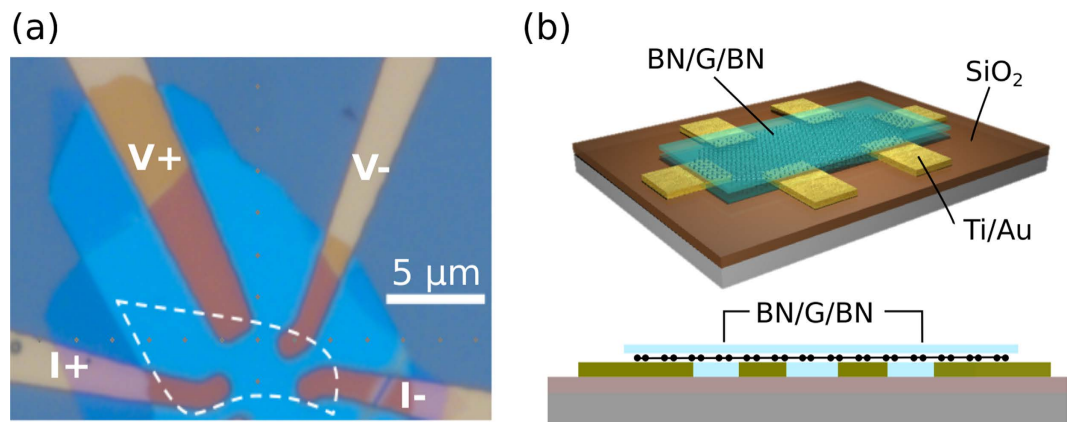
Figure 1. (a) Optical microscopy image of the sample with indicated current (I) and voltage (V) electrodes. The dotted white line indicates the position of the graphene flake and the light blue regions are the top and bottom h -BN sheets. (b) Schematic of the h -BN encapsulated graphene (BN/G/BN) device (top) and its cross-sectional view (bottom).
